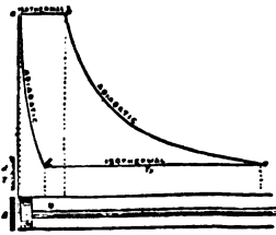
FIG. 9.—Carnot's Cycle with water and steam for working substance.
