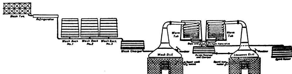
FIG. 7.—Diagram of Malt-whisky Pot-still Plant. (Messrs J. Buchanan's Gentaucher's Distillery, Speyside, N.B.)
