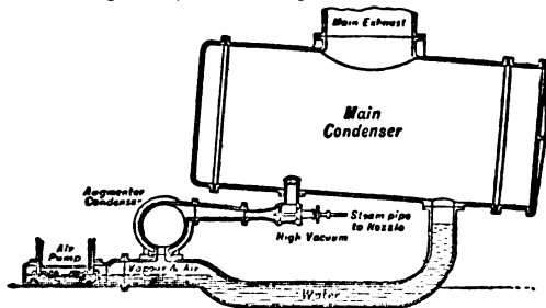
FIG. 68.—Parsons Vacuum Augmenter.
