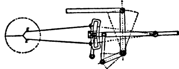
FIG. 30.—Gooch's Link-Motion.
