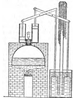
FIG. 8.—Leupold's Non-Condensing Engine, 1725.
