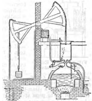
FIG. 4.—Newcomen's Atmospheric Engine, 1705.
