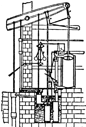
FIG. 7.—Watt's Double-Acting Engine, 1782.
