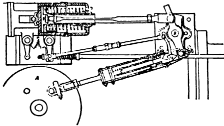
FIG. 46.—Corliss Valve-Gear, Spencer Inglis form.
