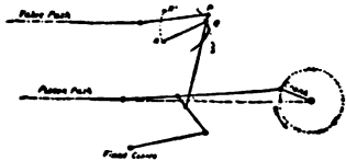
FIG. 35.—Diagram of Joy's Valve-Gear.
