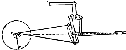
FIG. 31.—Allan's Link-Motion.
