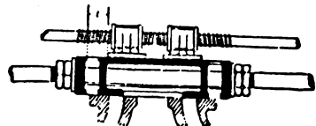
FIG. 37.—Expansion-Valve on back of Main Slide-Valve.
