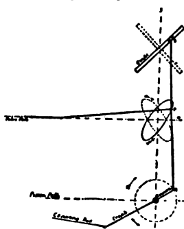
FIG. 33.—Hackworth's Valve-Gear.
