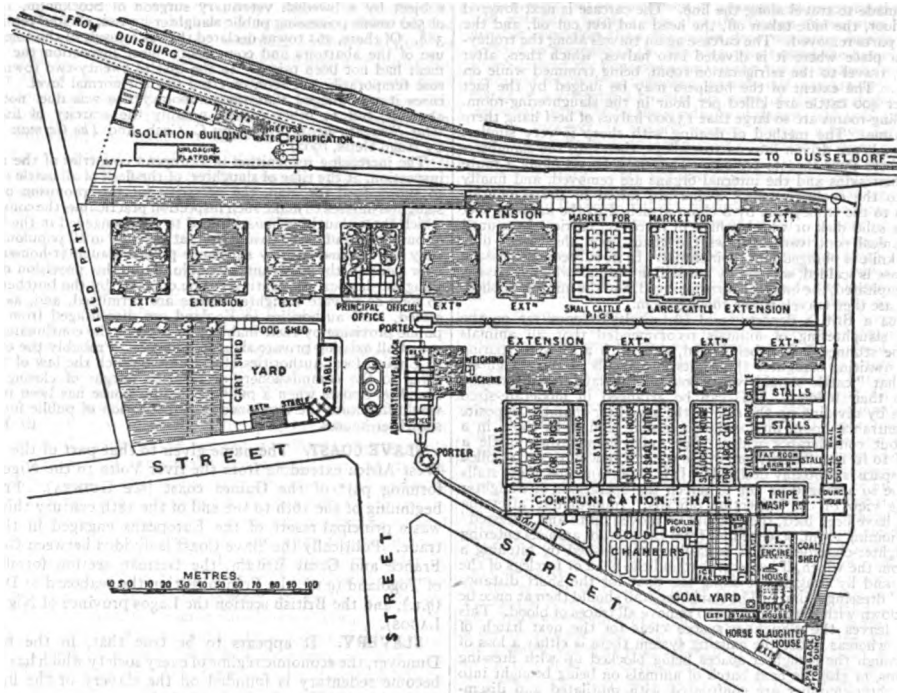
FIG. 2.—Plan of Public Slaughter-house and Cattle-market, Düsseldorf (1898).
