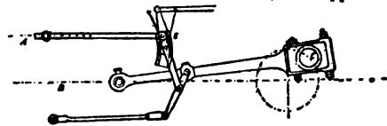
FIG. 36.—Joy's Gear as applied to a Locomotive.
