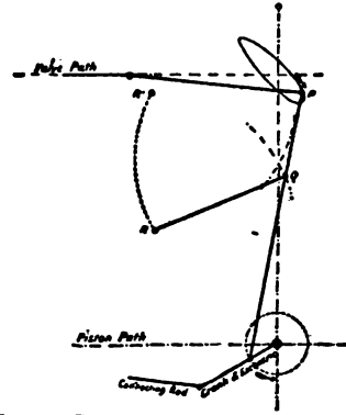
FIG. 34.—Bremme's or Marshall's Valve-Gear.
