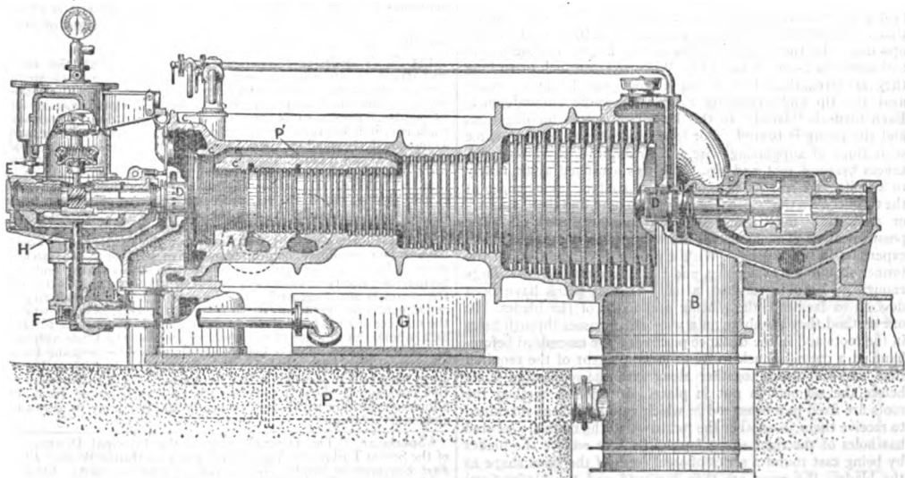
FIG. 60.—Parsons Turbine.
