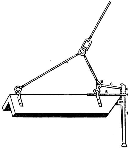
FIG. 3.—The Submarine Sentry.
