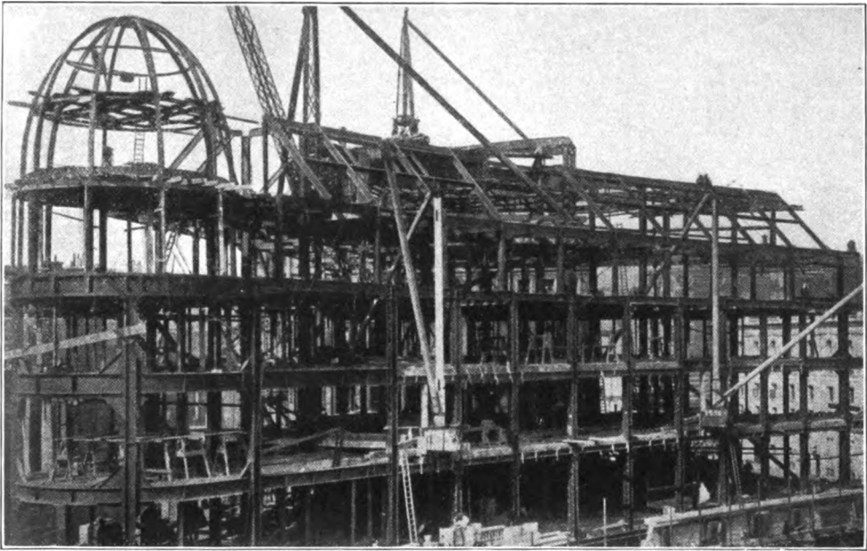
Fig. 1.—The Morning Post Building, London.
