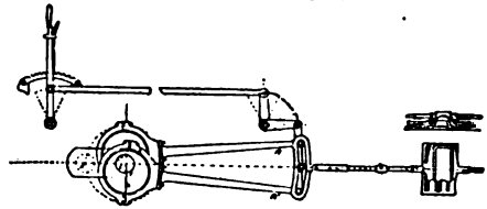
FIG. 29.—Stephenson's Link-Motion.
