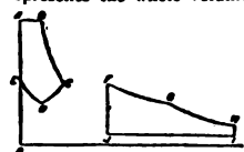
FIG. 17.—Compound Diagrams: Receiver type.
