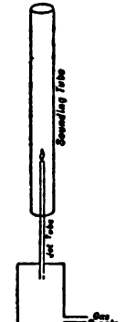
FIG. 40.—Singing Flame.
